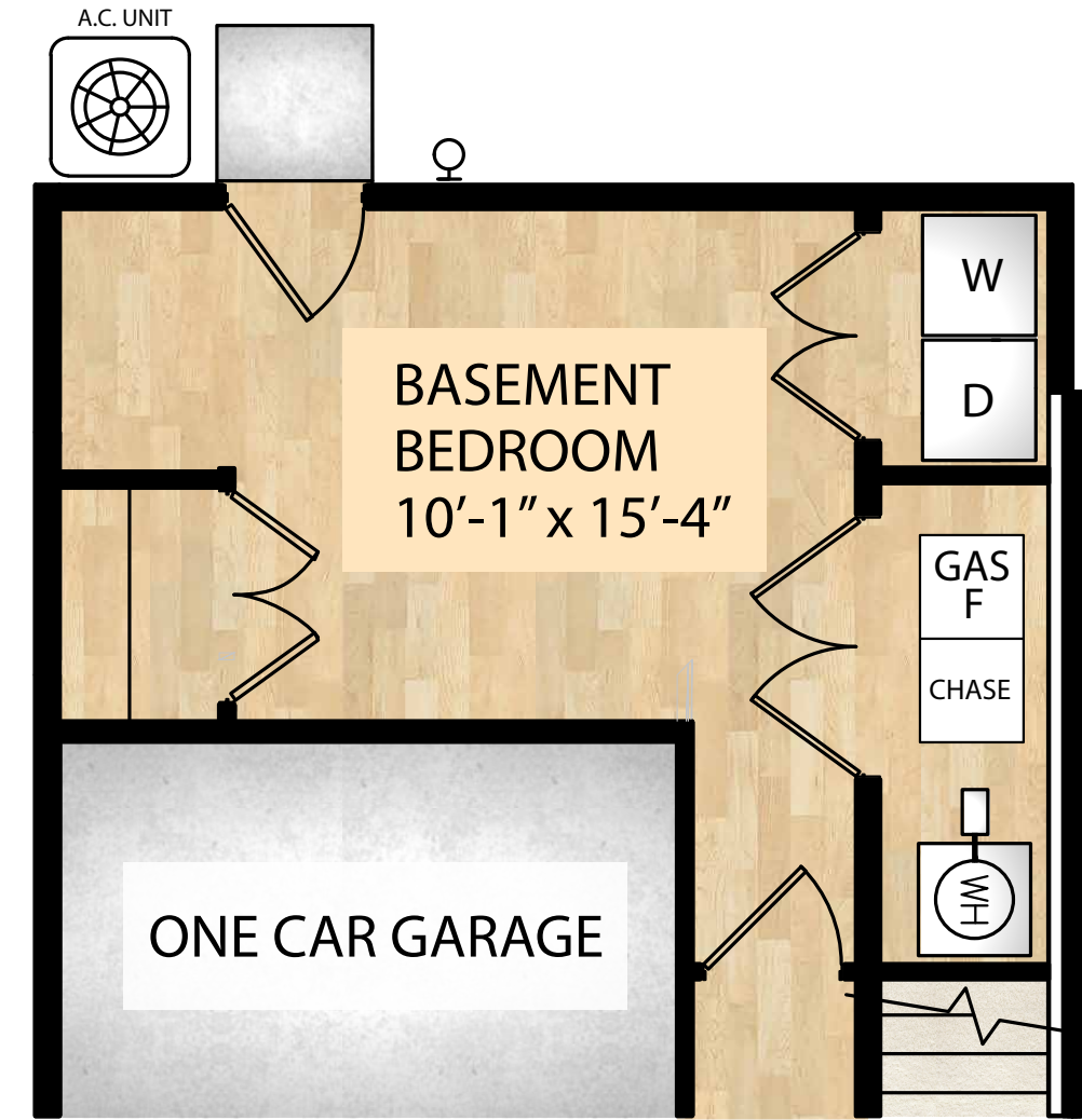
OPTIONAL BEDROOM & FINISHED LAUNDRY
